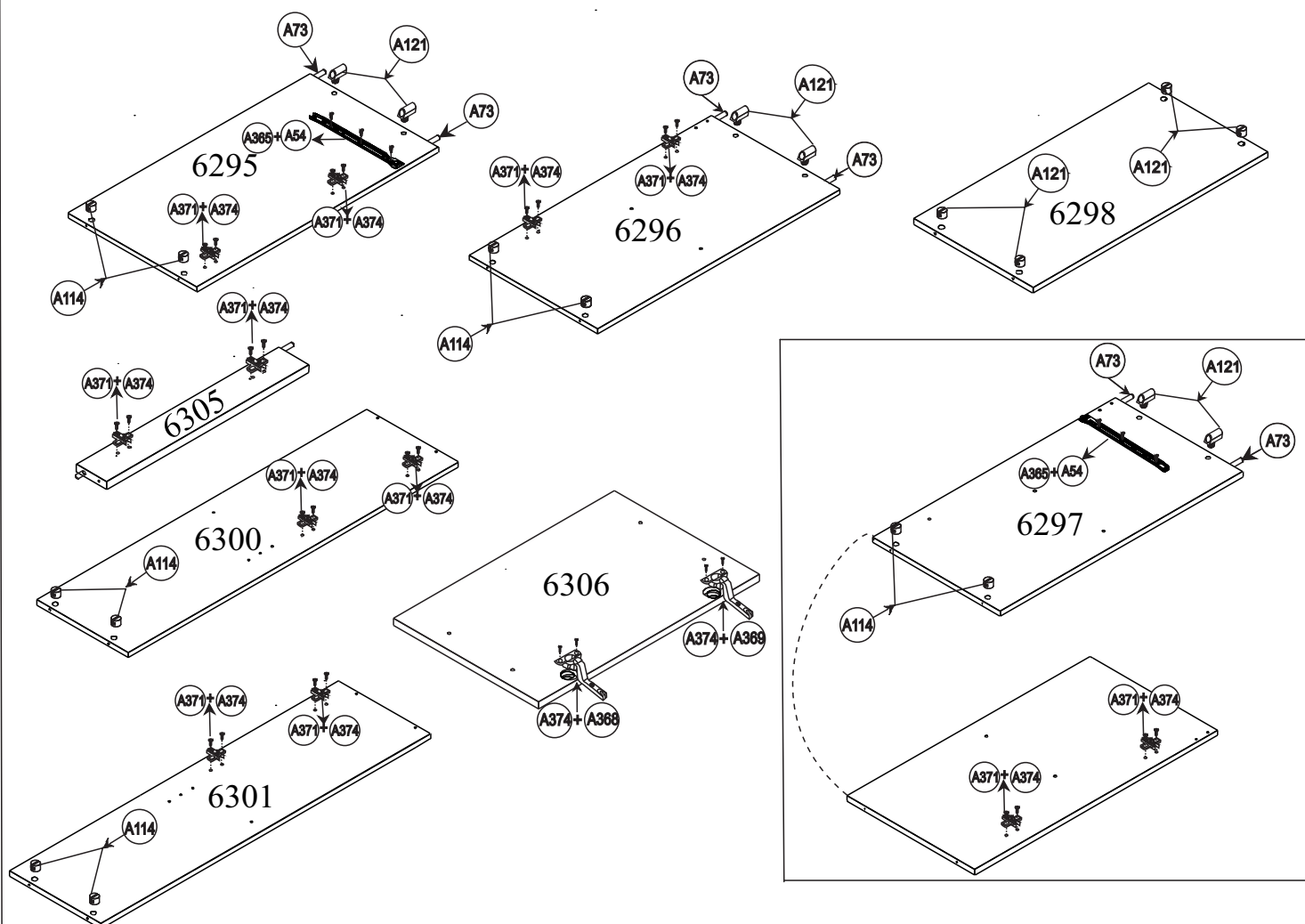
(A121 - Trapezio) (A073 - cavilha 6,0x30) (A54 - Parafuso 3,5x12 CC) (A092 - Cola) (A374 - Parafuso 3,5x12 CP)
